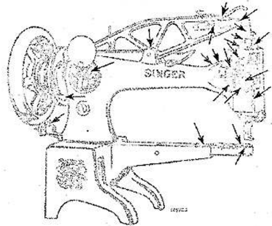
Fig. 3. Oiling Rear of Machine
